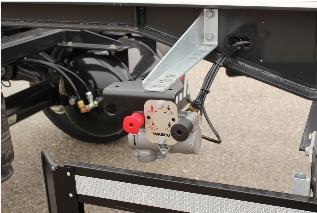
Stop support at front, tiltable and relocatable
